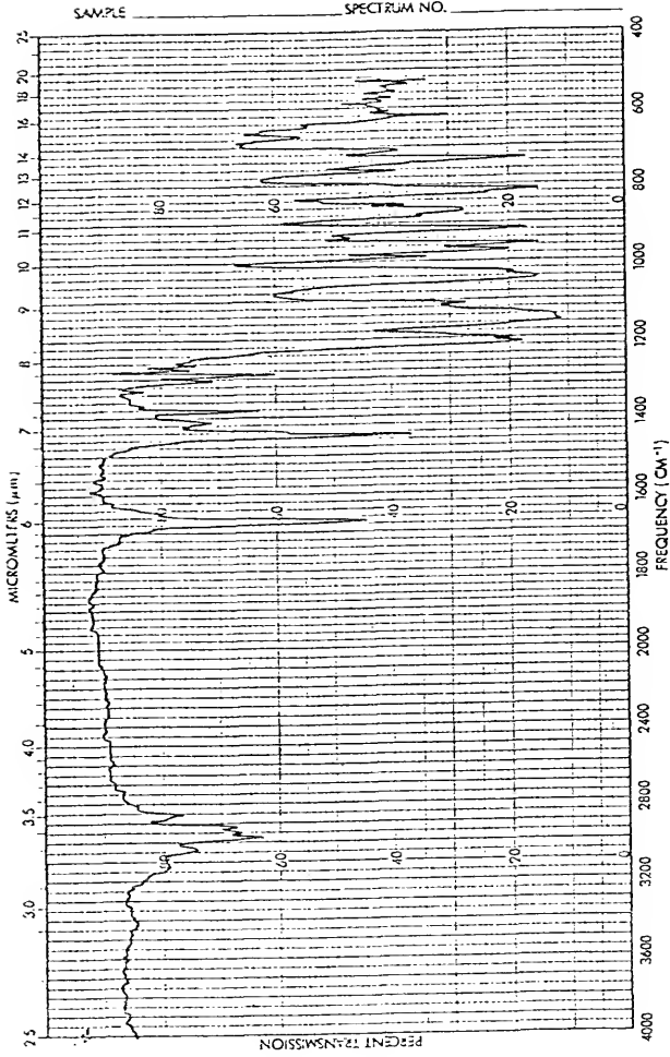
Figure 13 -- Infrared of \text{CF}_2\text{BrCFClCH}=\text{CHCl}_3
